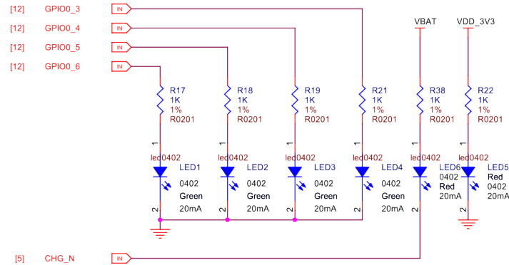
Fig. 3.37: LED indicators
