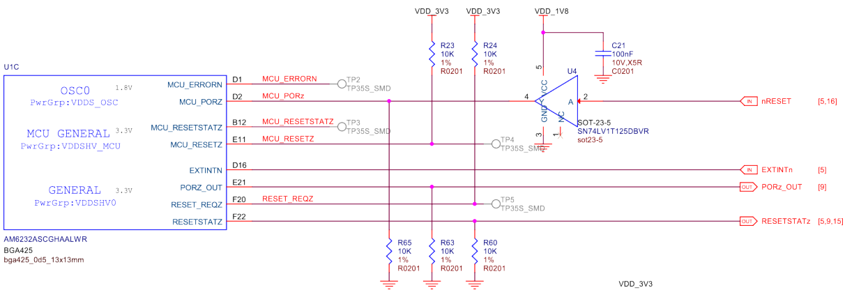
Fig. 3.20: MCU system
