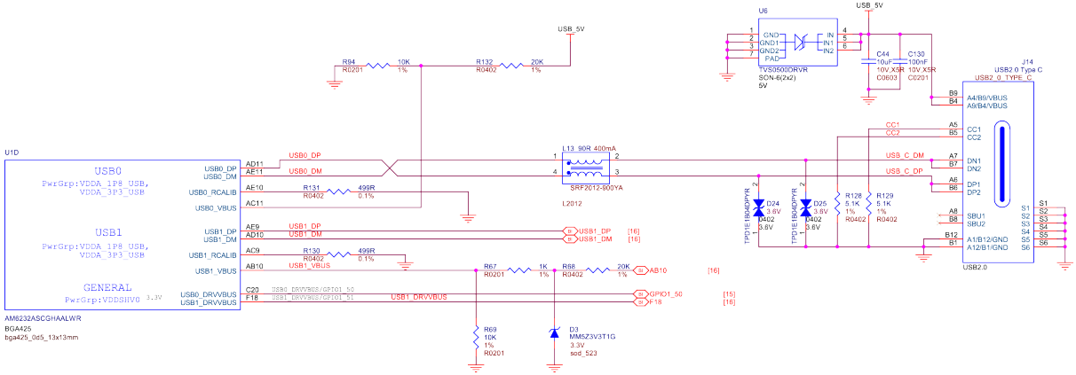
Fig. 3.31: USB connections
