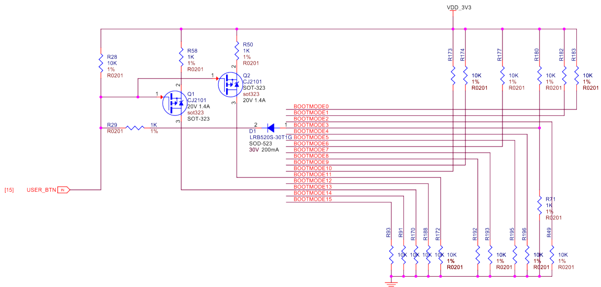
Fig. 3.11: Bootstrap pins connection
