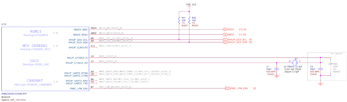
Fig. 3.21: Wakeup domain
